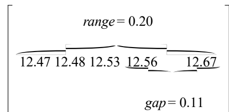
Figure 31. Diagram showing the range and gap of a series of data points.
